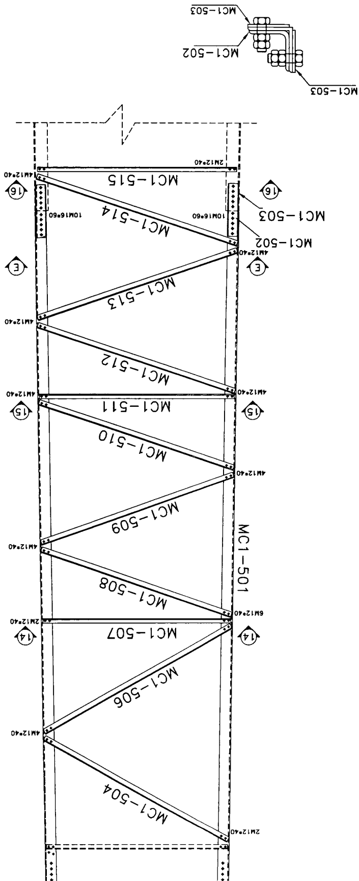
SEC. E-E
