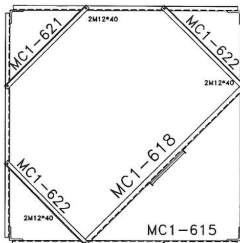
SEC. 19-19
