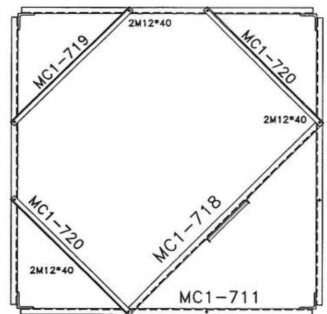
SEC. 21-21
