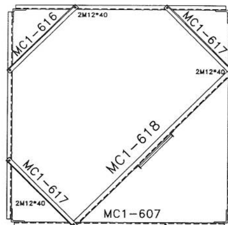
SEC. 17-17
