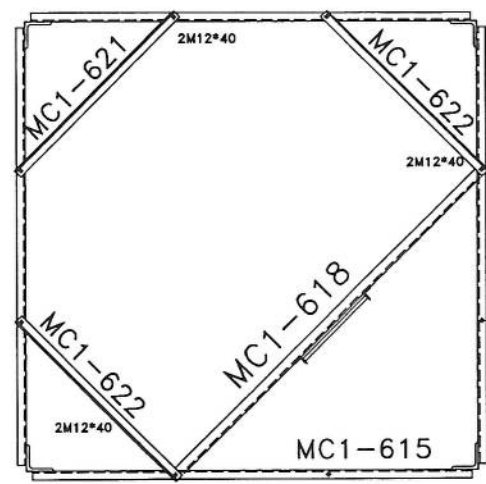
SEC. 19-19
