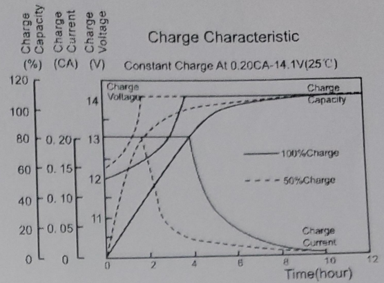
Battery Voltage Vs. Charge Time
