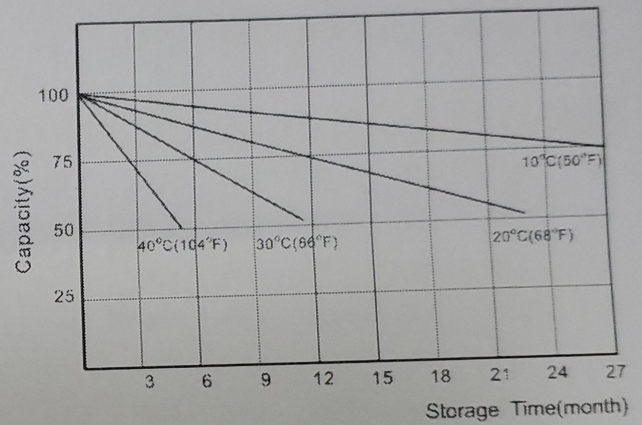
Capacity Retention Characteristic
