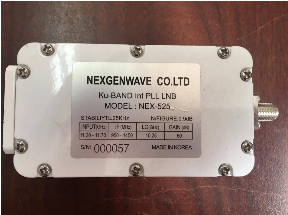
Figure 4: Specifications of the LNB used in the remote sites.
