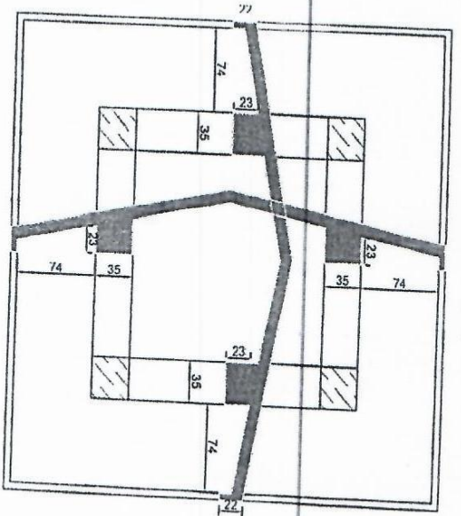
Roof shuttering plan
