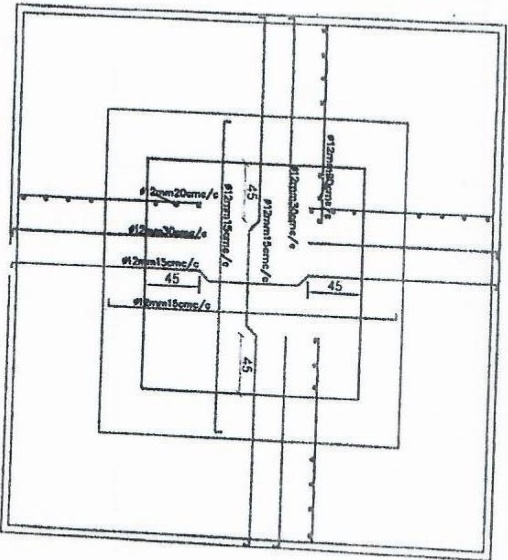
First floor Slab steel plan
