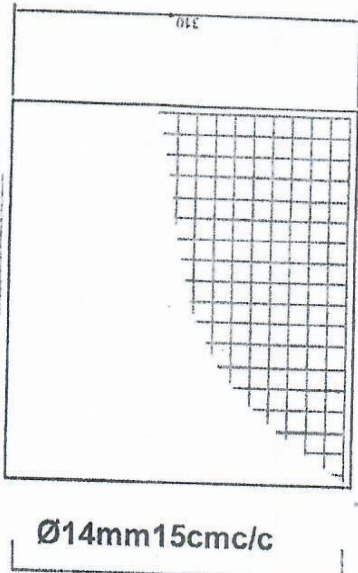
Foundation plan
