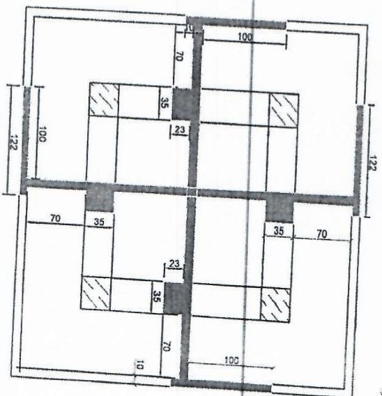
First floor Slab shuttering plan
